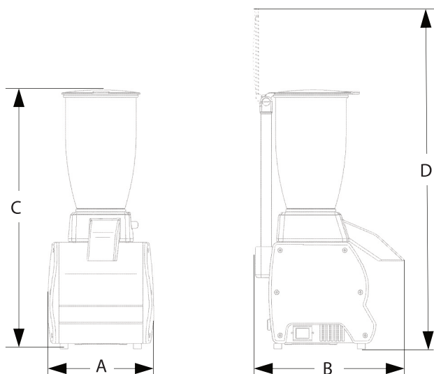
FIG. n°2 - Overall dimensions
